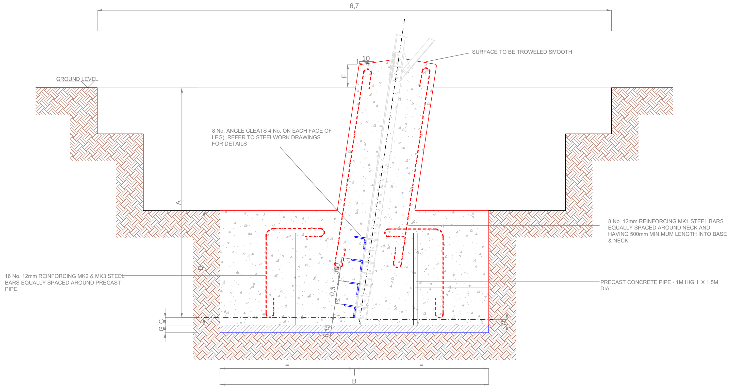
FOUNDATION ELEVATION SECTION
